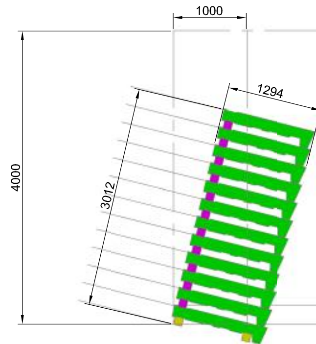
SECTIONAL VIEW
